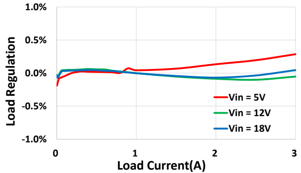
Figure 4. Load Regulation vs Load Current ( V_{OUT}=3.3V, L=1.5\mu H )
