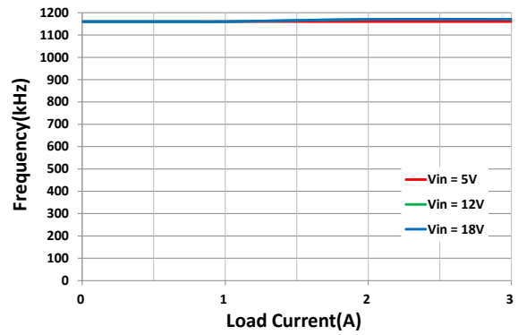
Figure 8. Frequency vs Load Current ( V_{OUT}=3.3V , L=1.5\mu H )
