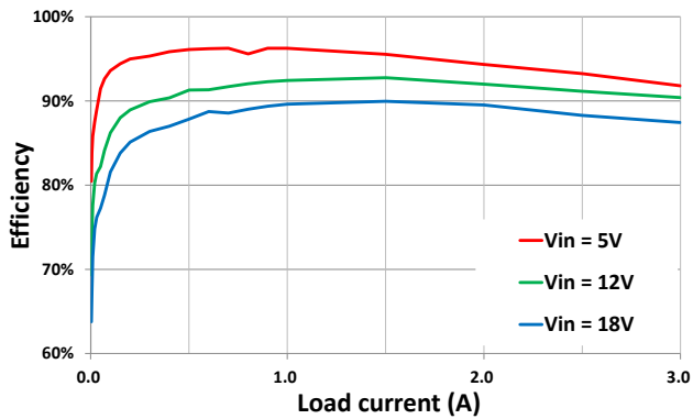
Figure 1. Efficiency vs. Load Current ( V_{OUT}=3.3V, L=1.5\mu H )
