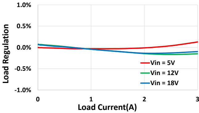
Figure 9. Load Regulation vs Load Current ( V_{OUT}=3.3V , L=1.5\mu H )
