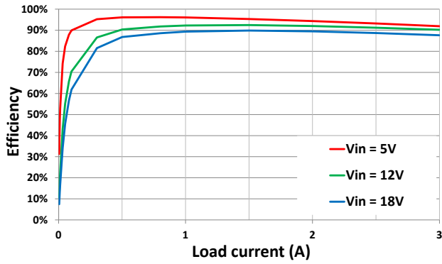
Figure 7. Efficiency vs. Load Current ( V_{OUT}=3.3V , L=1.5\mu H )
